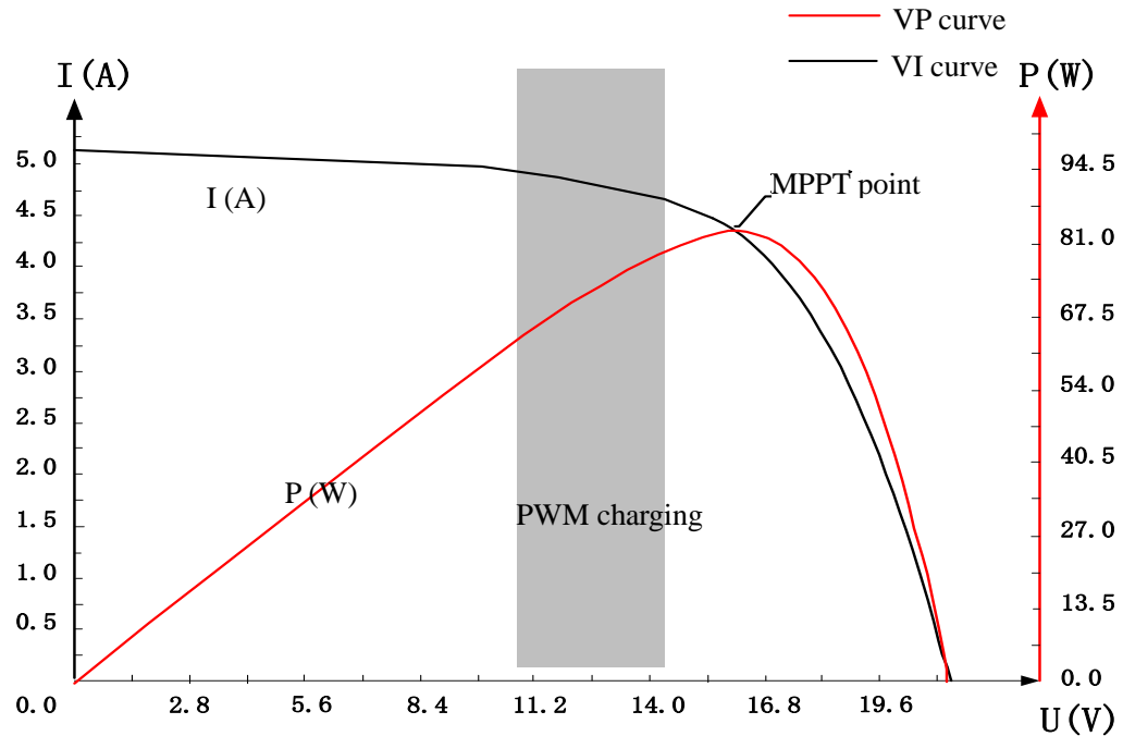
Fig. 1-2 Solar panel output characteristic curve
